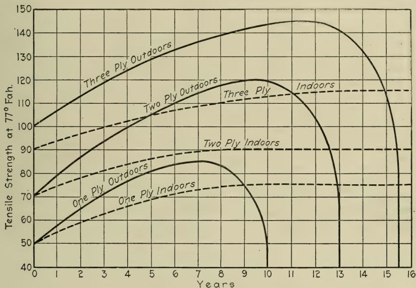
FIG. 208.—Tensile Strength Curves of Prepared Roofings on Exposure.
